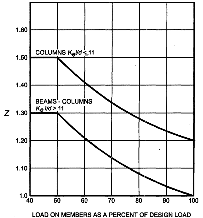
FIGURE 721.6.3(1) LOAD FIGURE
