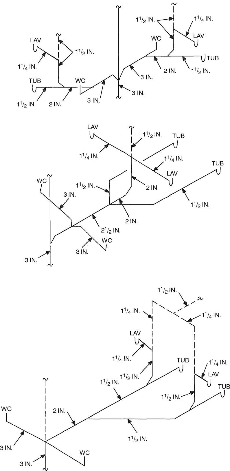
FIGURE N2 TYPICAL DOUBLE-BATH WET-VENT ARRANGEMENTS
