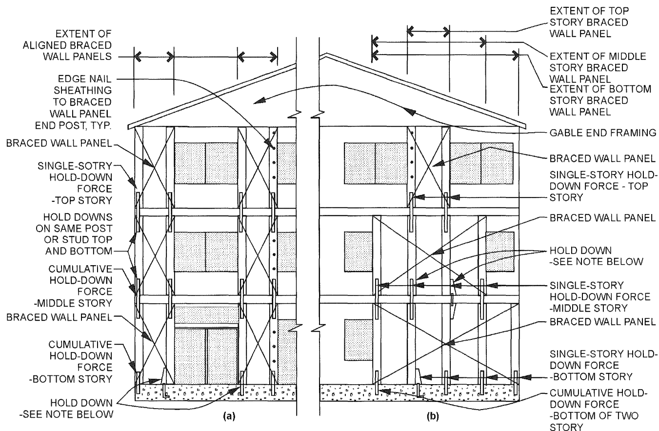
(a) Braced wall panels stacked (aligned story to story) Use cumulative hold-down force. (b) Braced wall panels mixed stacked and not stacked. Use hold-down force as noted.
