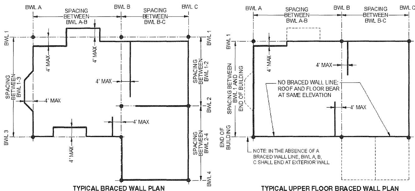
FIGURE R602.10.1.1 BRACED WALL LINES
