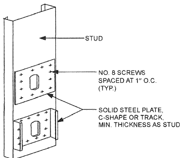
FIGURE R603.2.5.3 STUD WEB HOLE PATCH
