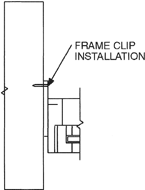
FIGURE R612.7.2(2) FRAME CLIP
